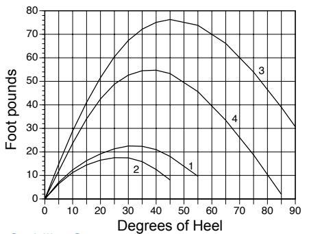
Stability Curves
