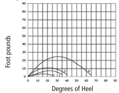
Stability Curves
