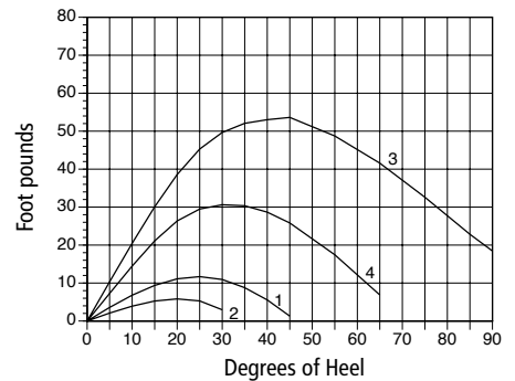
Stability Curves
