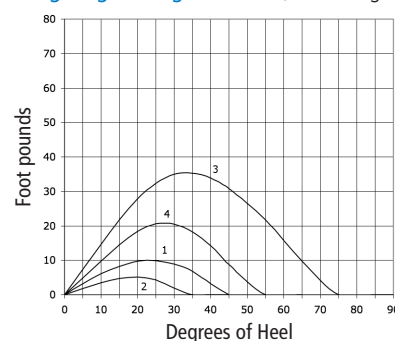
Stability Curves
