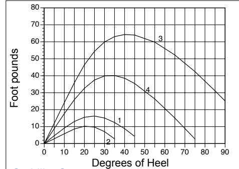
Stability Curves
