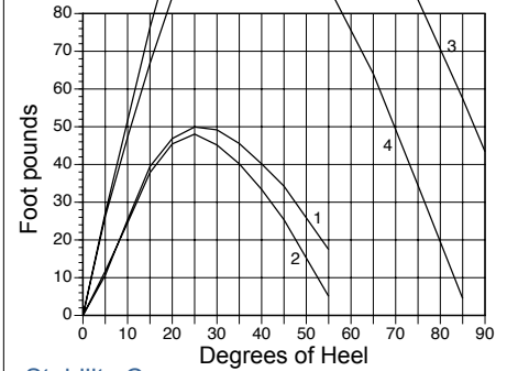
Stability Curves
