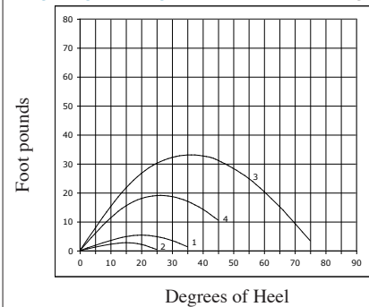
Stability Curves
