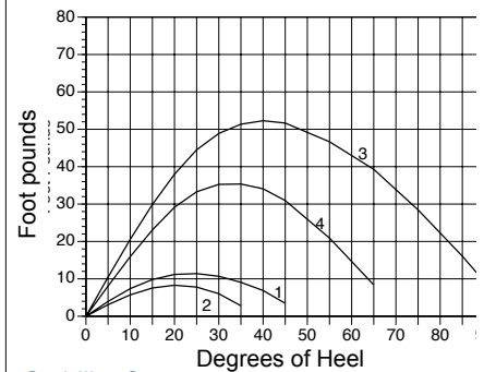
Stability Curves
