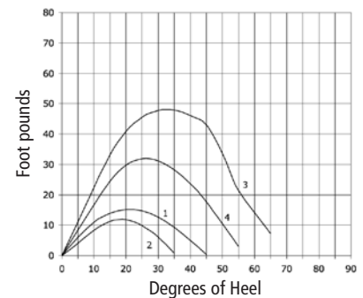
Stability Curves
