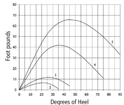
Stability Curves
