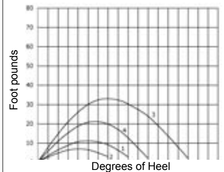
Stability Curves
