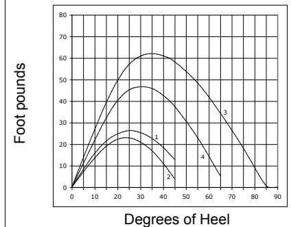
Stability Curves
