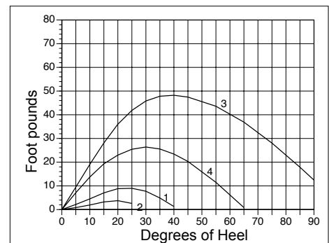
Stability Curves
