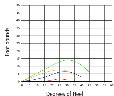
Stability Curves*
