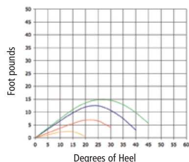
Stability Curves*
