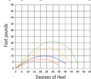
Stability Curves*
