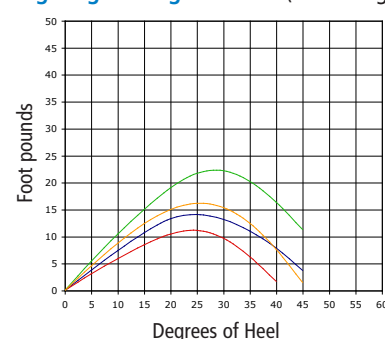
Stability Curves*
