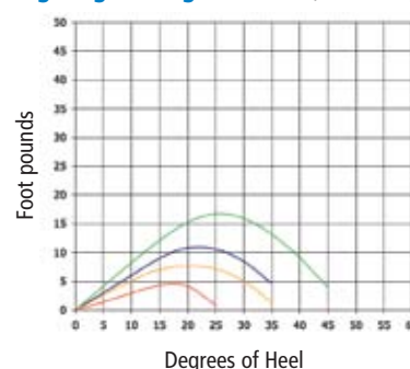
Stability Curves*
