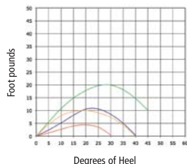
Stability Curves*
