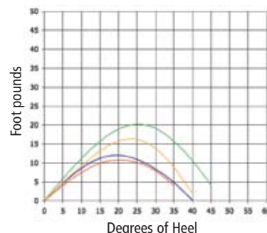
Stability Curves*
