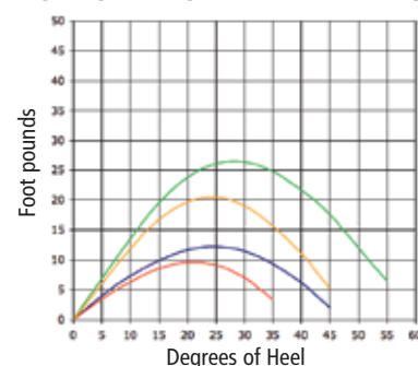
Stability Curves*
