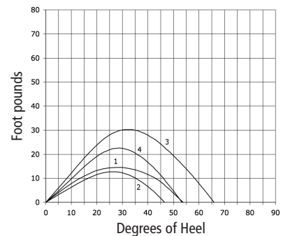
Stability Curves
