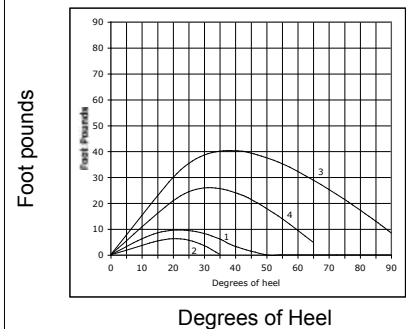
Stability Curves
