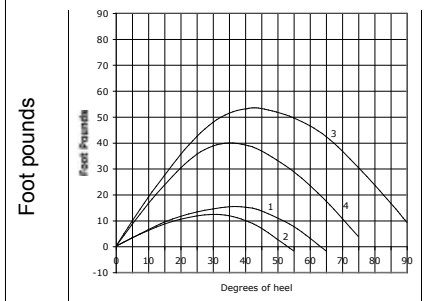
Righting/Heeling Moments (Fixed-weight)
