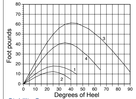
Stability Curves
