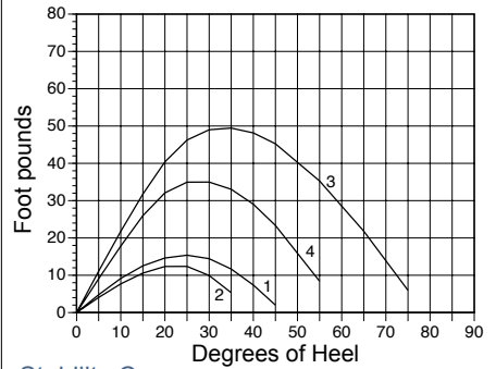
Stability Curves
